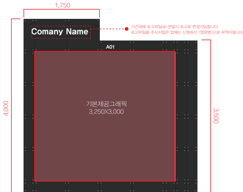
▲ FORNT VIEW
